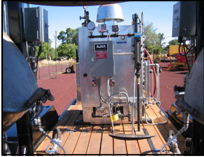
A 10 HP STEAM BOILER IS INCLUDED TO OPERATE THE NEWHOUSE ESSENTIAL OIL STILLS
